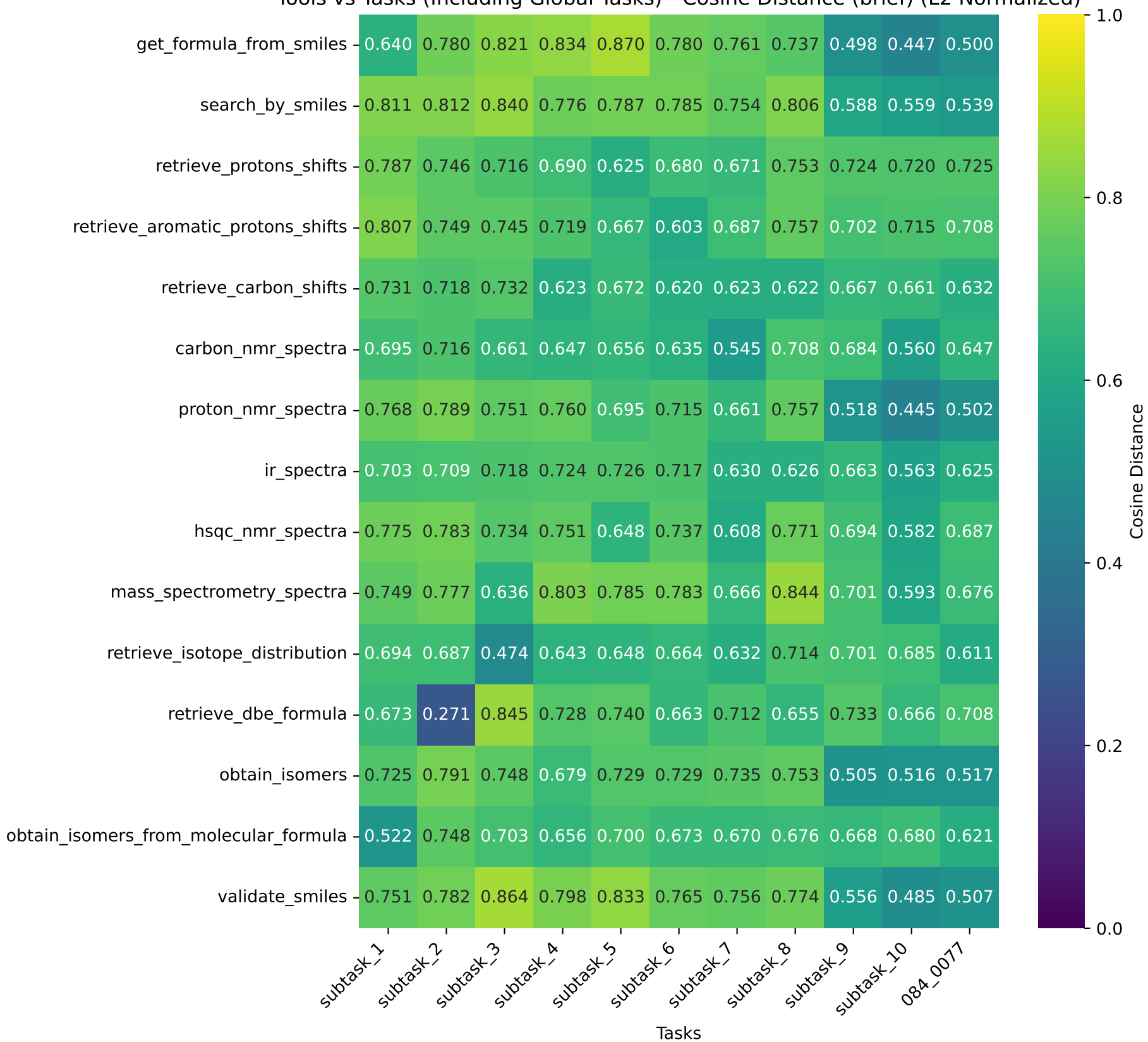
Tools vs Tasks (Including Global Tasks) - Cosine Distance (brief) (L2 Normalized)
