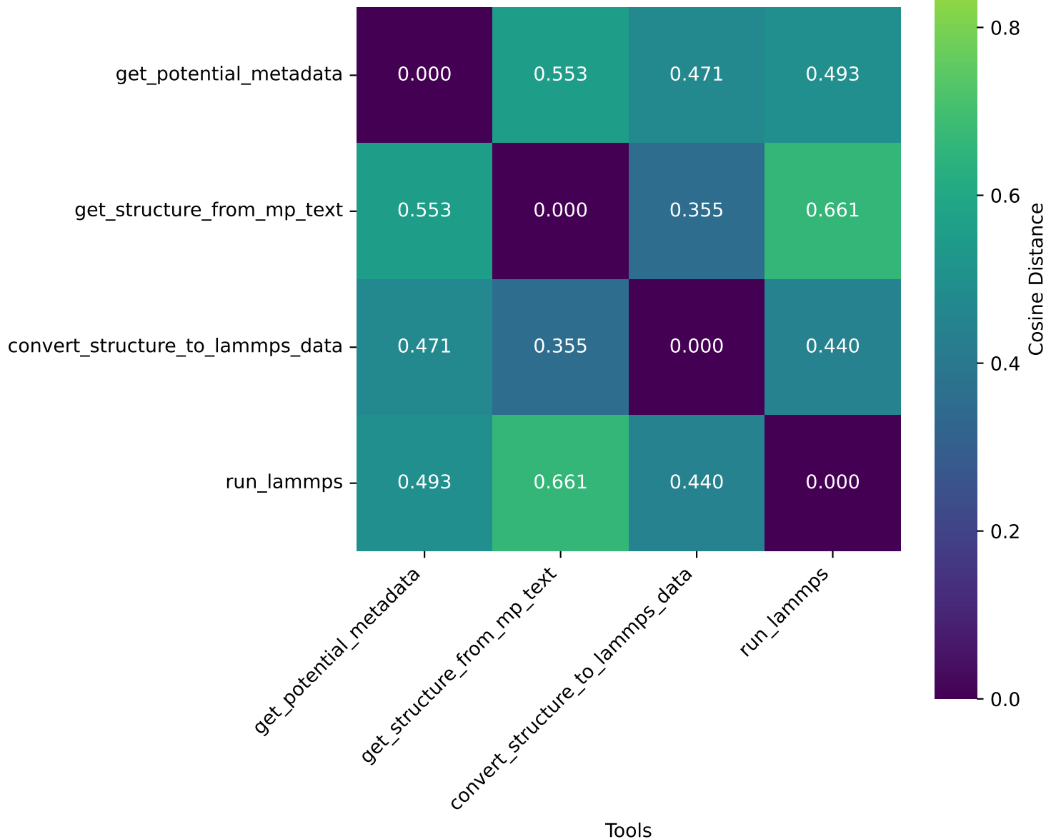
Tools vs Tools - Cosine Distance (workflow) (L2 Normalized)
