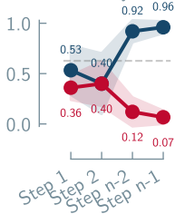
Inorganic Qualitative Analysis
