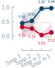
Retrosynthetic Planning
