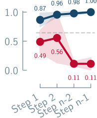
Circuit Inference
