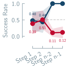
Spectroscopic Structure Elucidation
