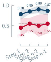
ML-based Property Prediction
