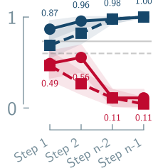
Circuit Inference
