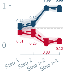
Retrosynthetic Planning
