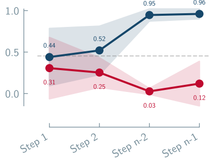
Retrosynthetic Planning
