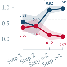
Inorganic Qualitative Analysis
