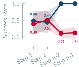
Spectroscopic Structure Elucidation
