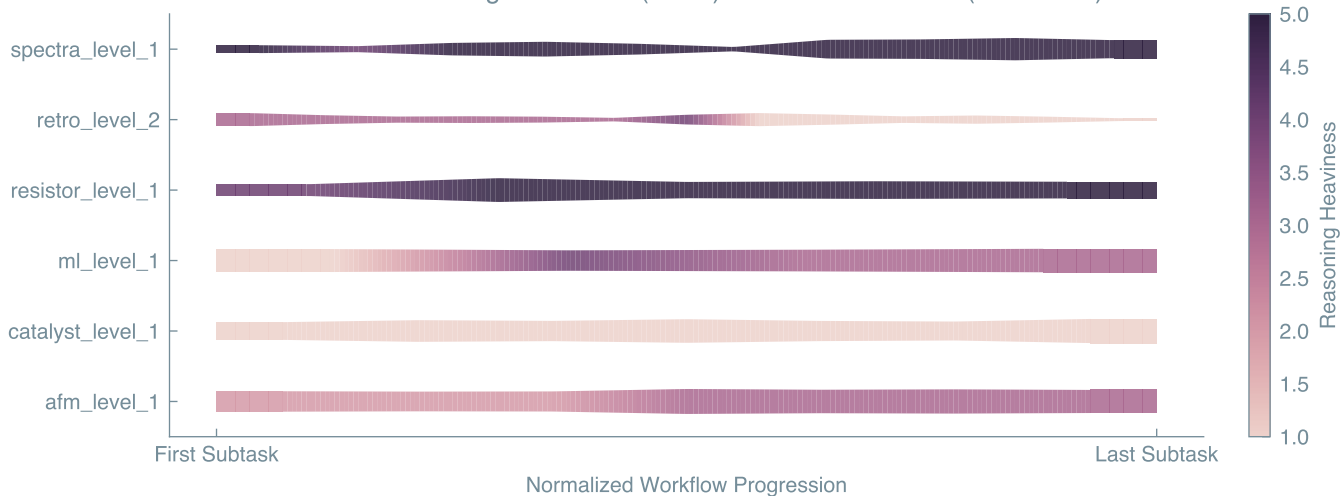
Subtask Reasoning Heaviness (Color) and Success Score (Thickness)
