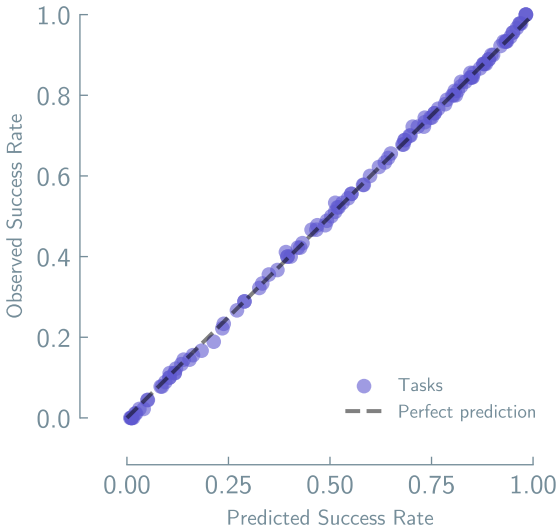
Task-Averaged LOO Predictions
