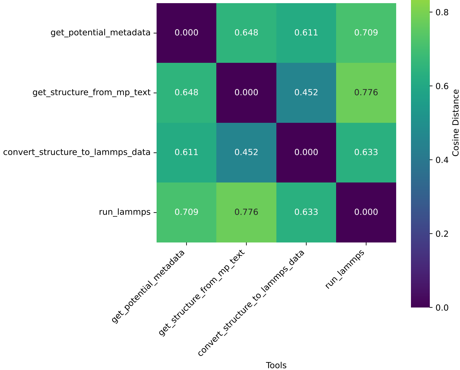
Tools vs Tools - Cosine Distance (brief) (L2 Normalized)
