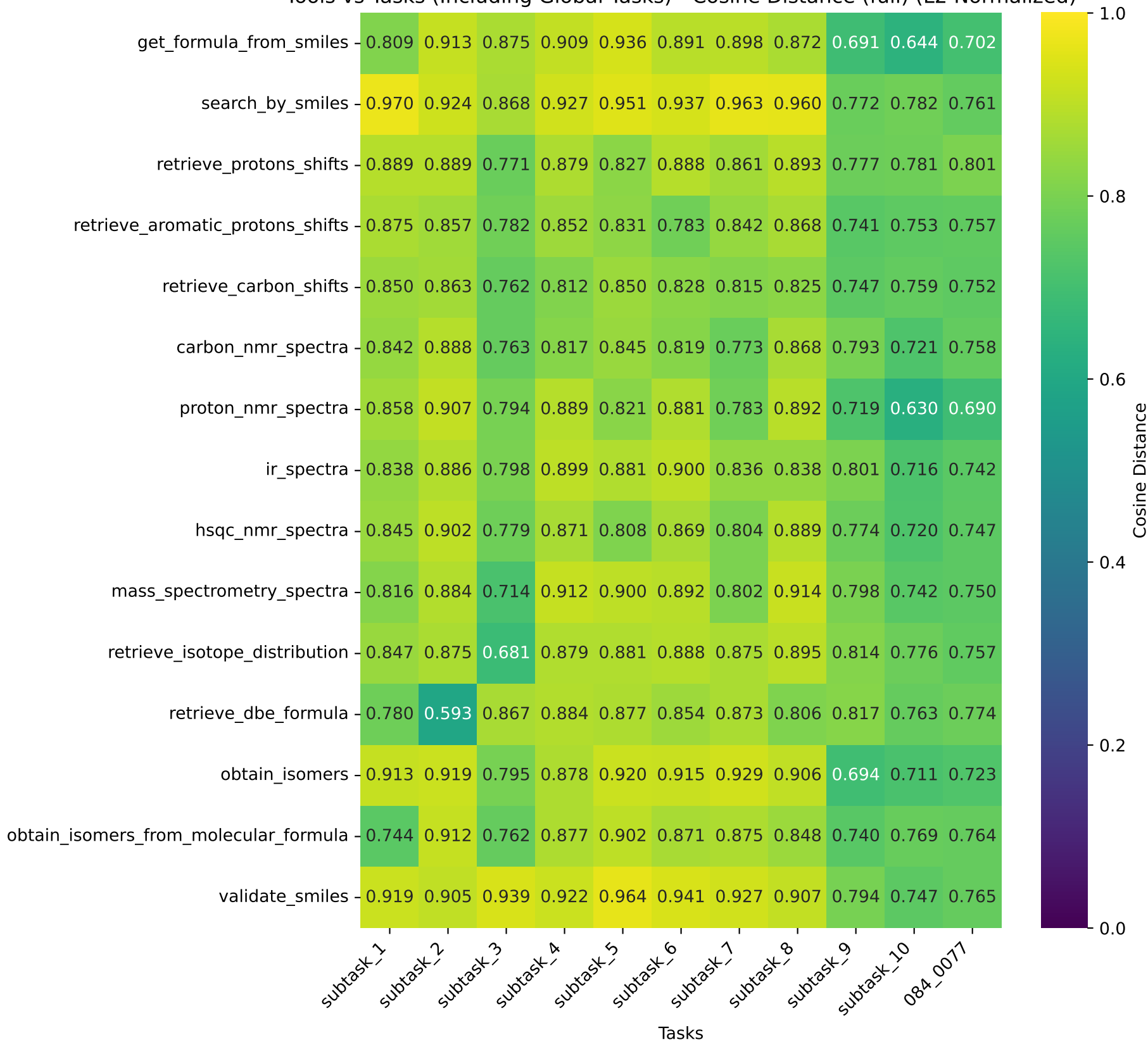
Tools vs Tasks (Including Global Tasks) - Cosine Distance (full) (L2 Normalized)
