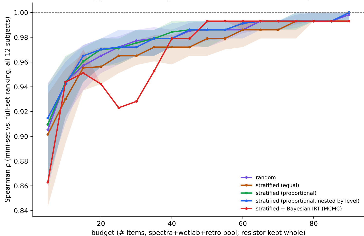
Global ranking preservation vs. budget — median \pm IQR over 200 draws/boots per method
