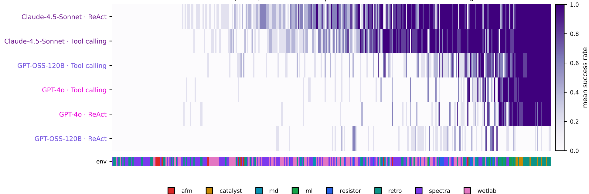
Sorted response matrix (6 model×scaffold subjects × 345 items) rows: best subject top → worst bottom | columns: easiest item left → hardest right
