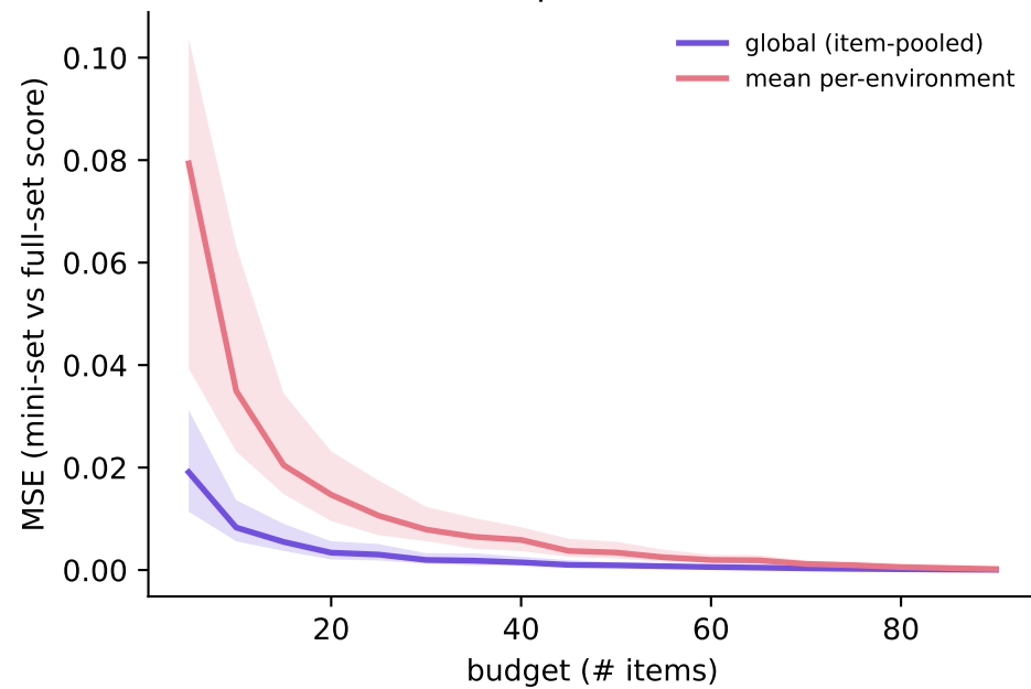
Score preservation
