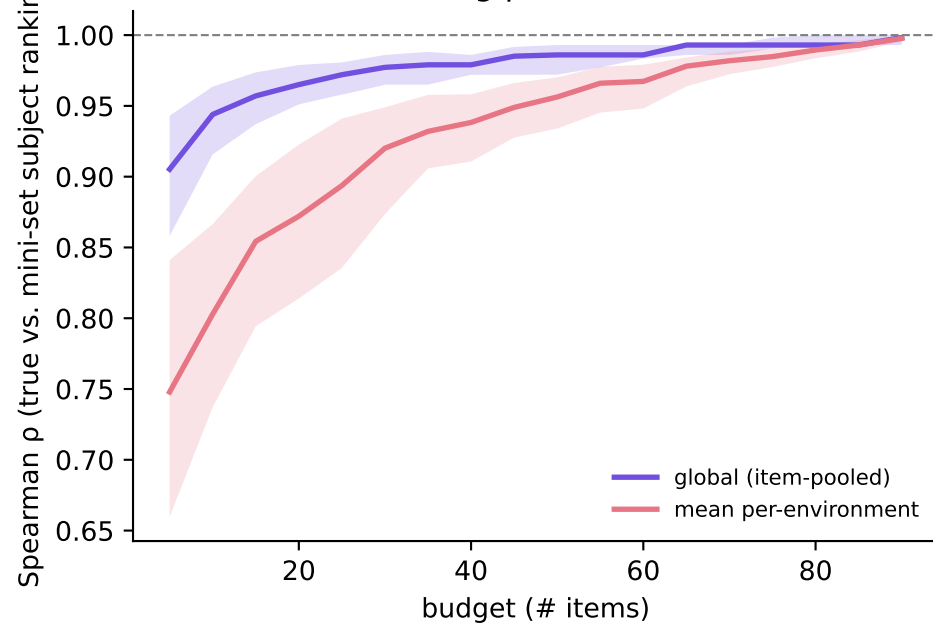
Ranking preservation
