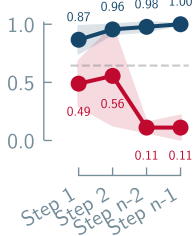
Circuit Inference
