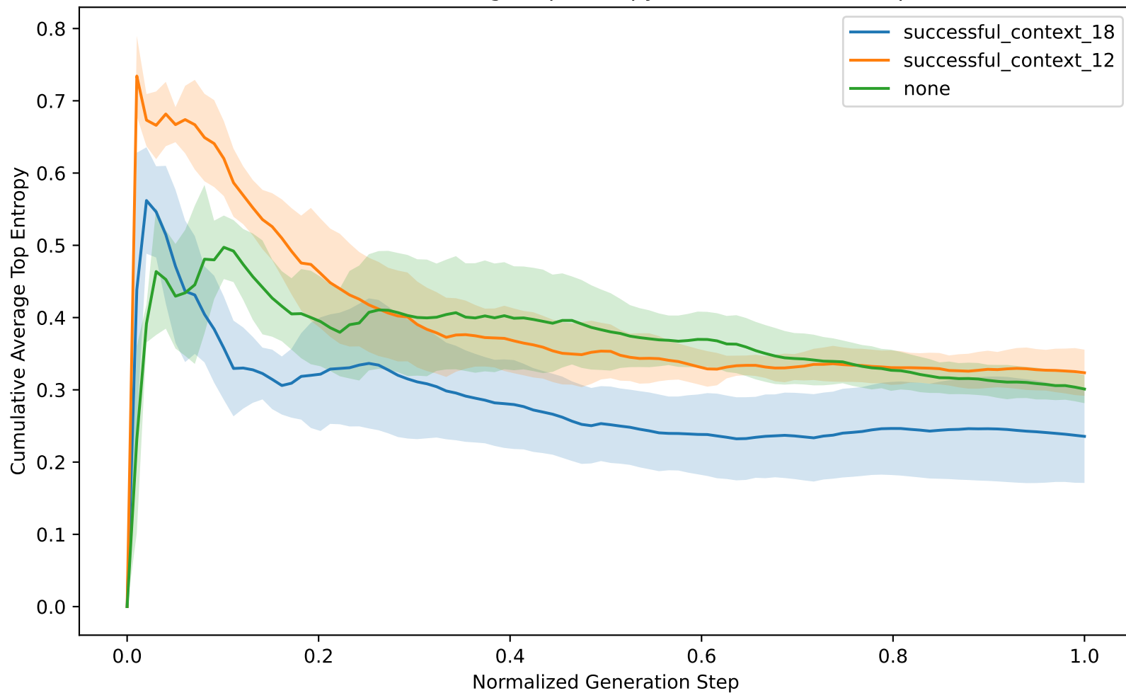
Cumulative Average Top Entropy Over Generation Steps
