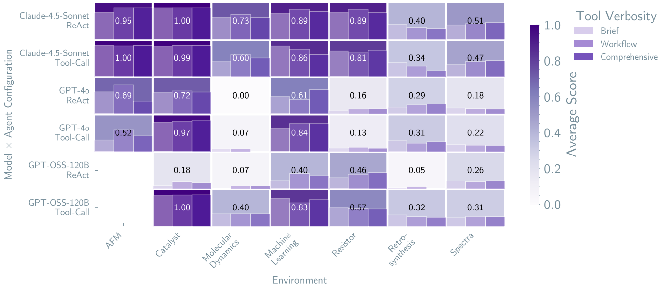
Performance with Verbosity Breakdown: 6 Configs × 7 Environments
