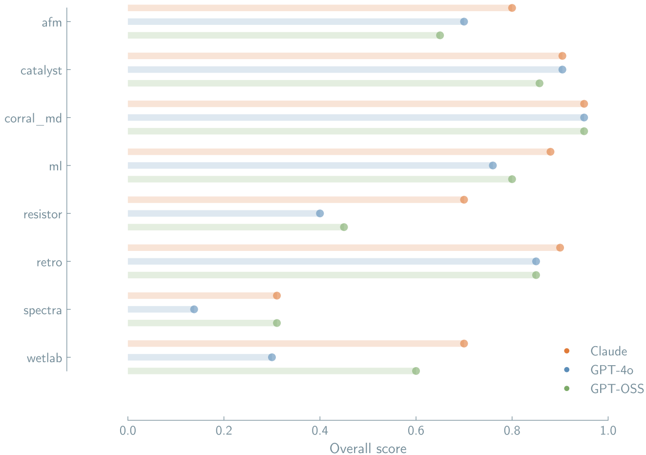
Reasoning QA scores
