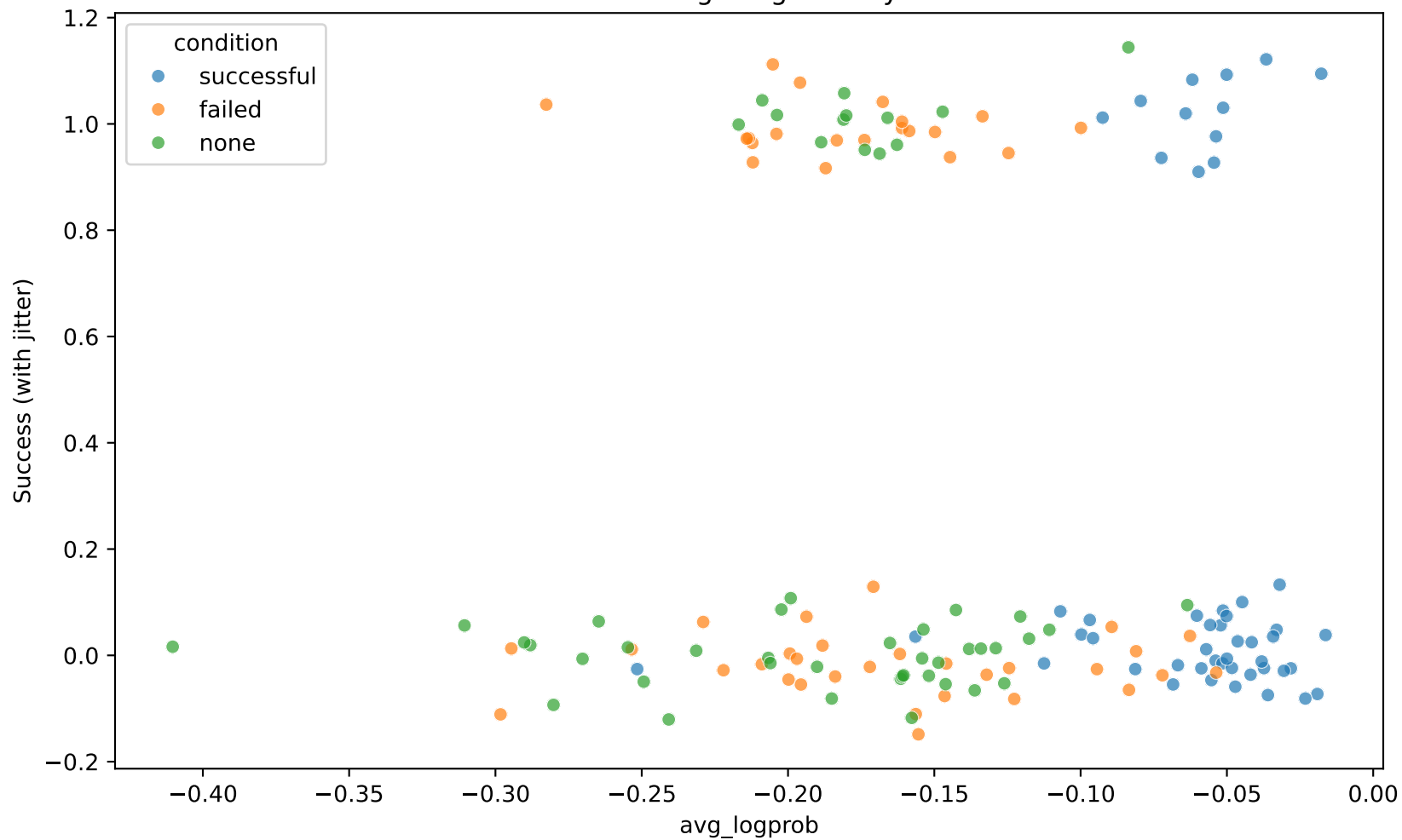
Success vs Average Log Prob by Condition
