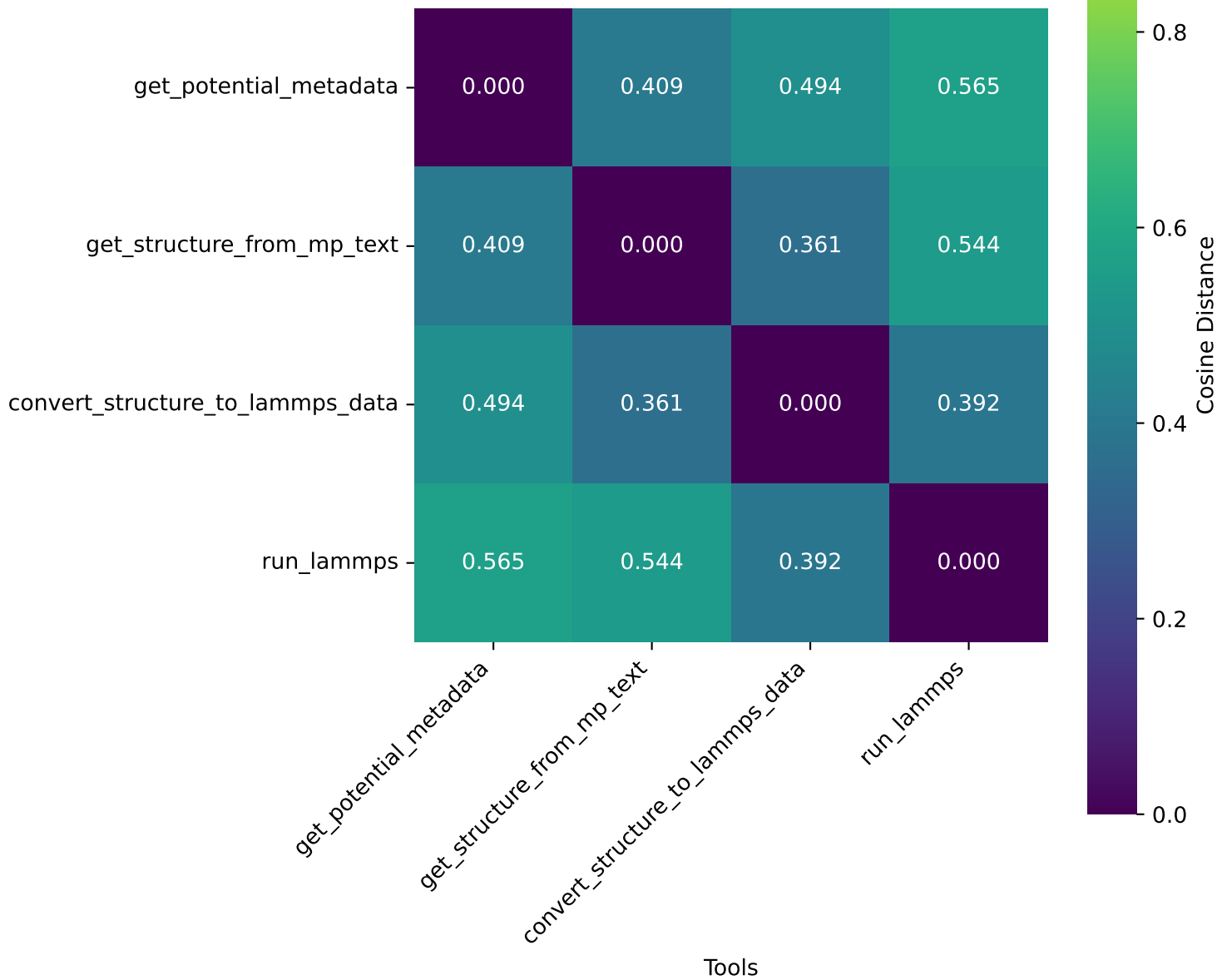
Tools vs Tools - Cosine Distance (full) (L2 Normalized)
