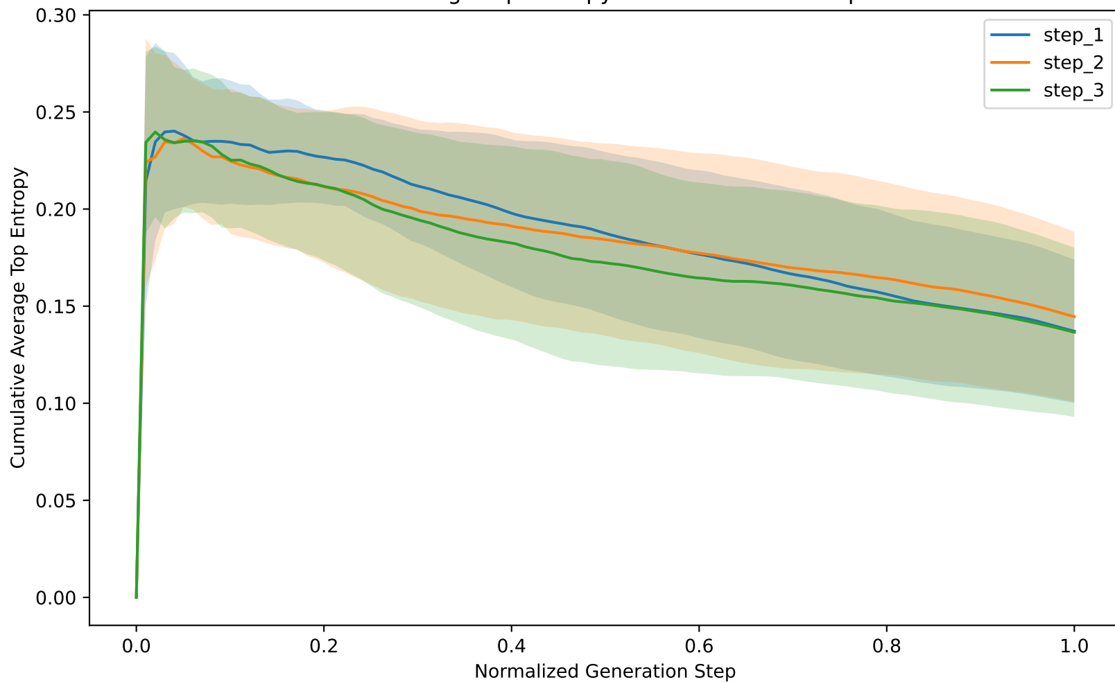
Cumulative Average Top Entropy Over Generation Steps - Failed
