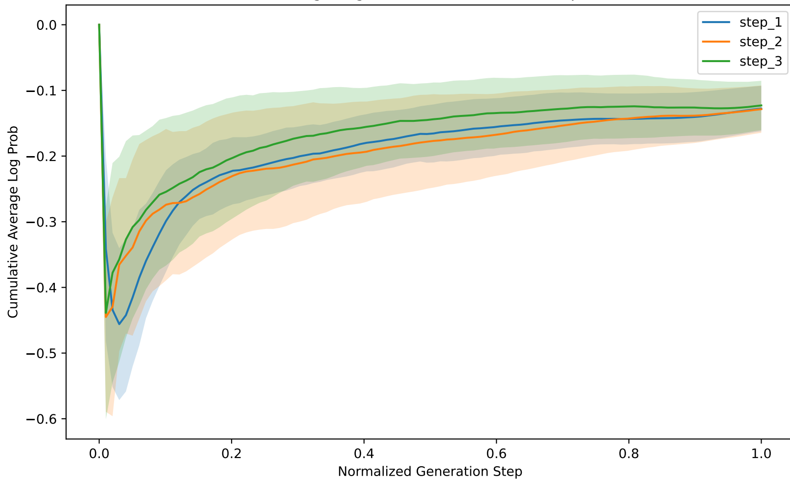
Cumulative Average Log Prob Over Generation Steps - Successful
