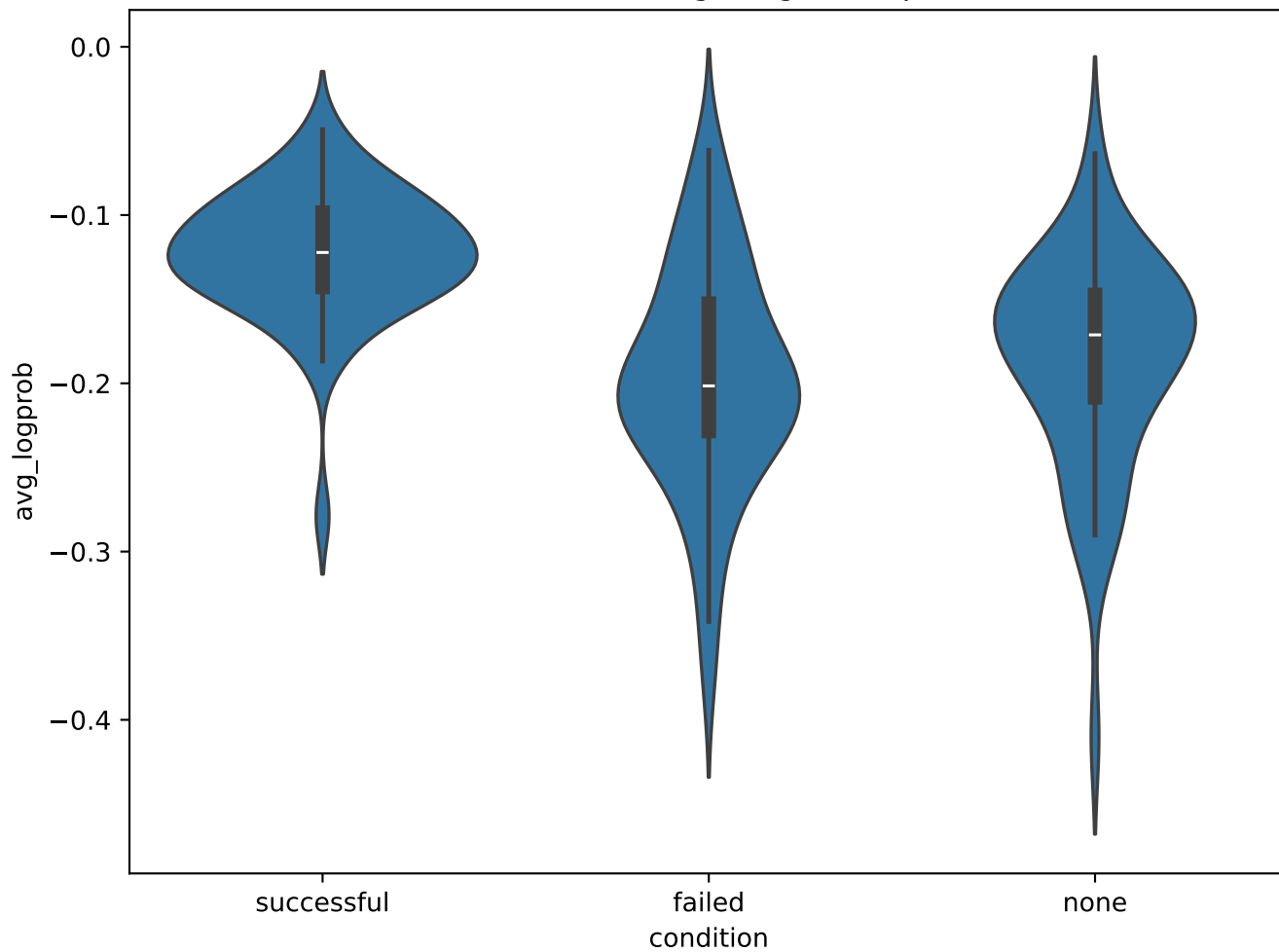
Distribution of Average Log Probs per Trace
