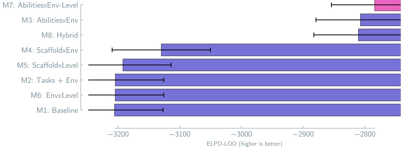
Model Comparison (Binomial)
