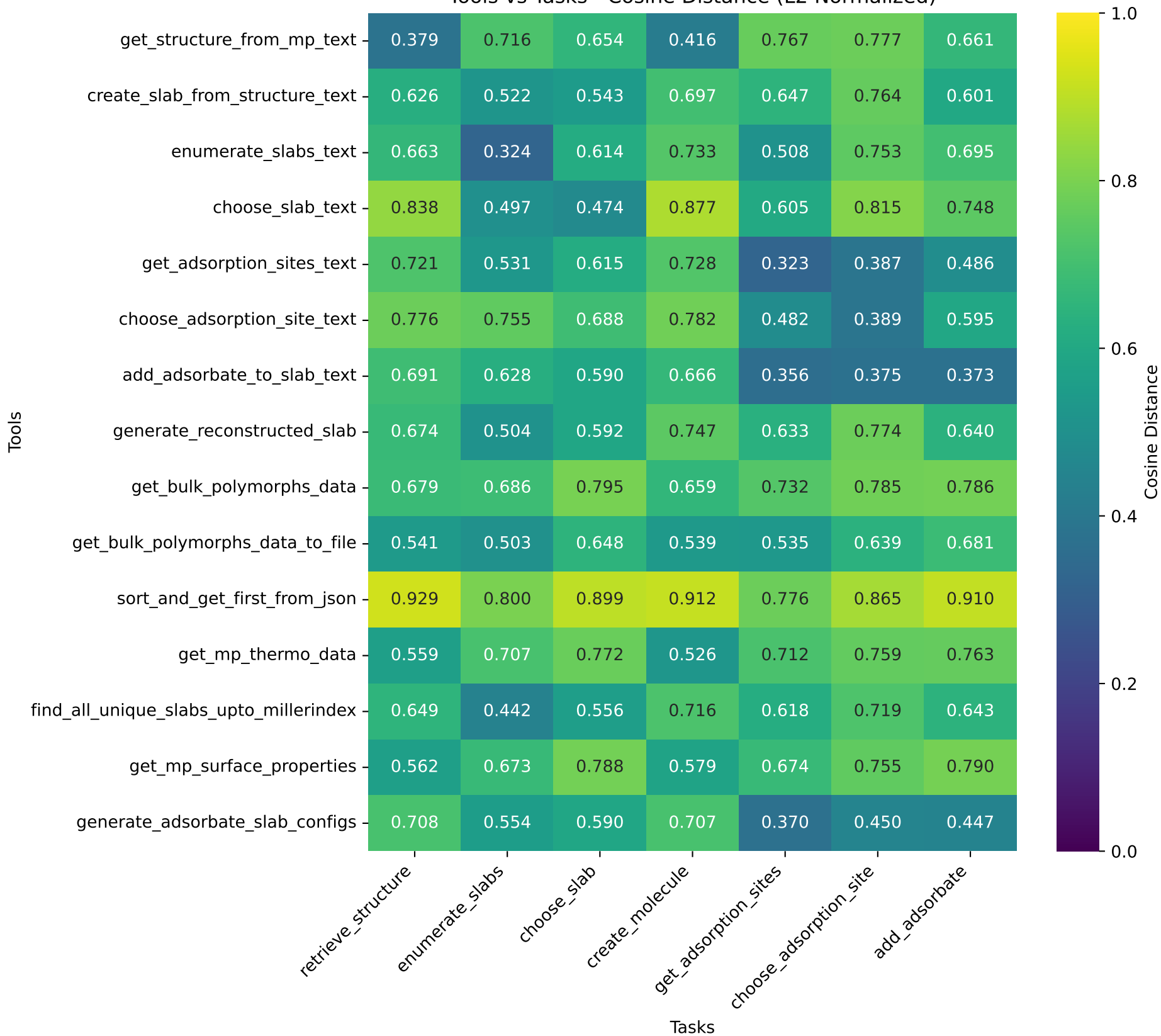
Tools vs Tasks - Cosine Distance (L2 Normalized)
