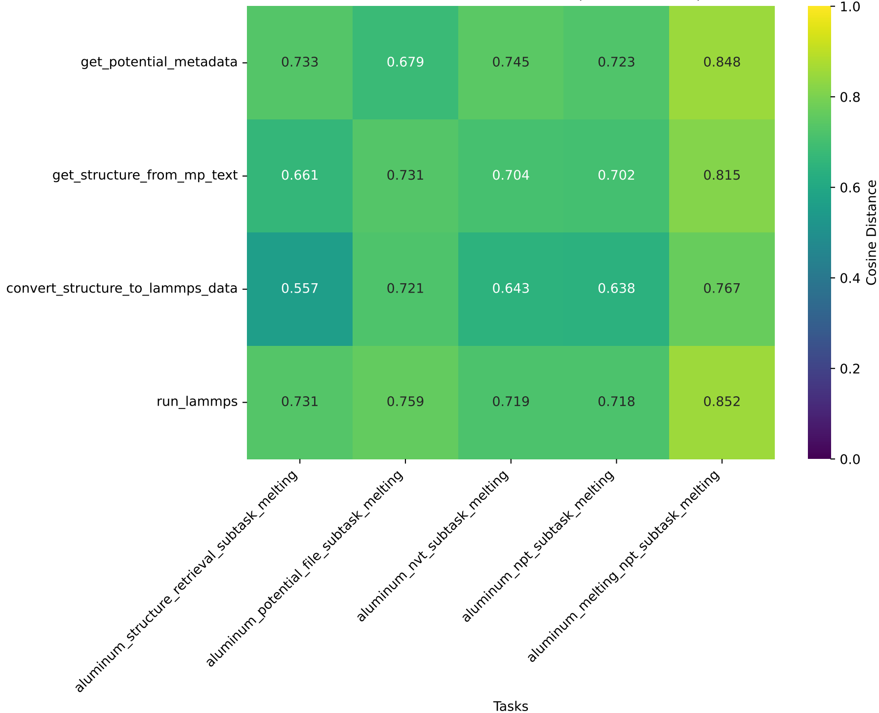
Tools vs Tasks - Cosine Distance (L2 Normalized)
