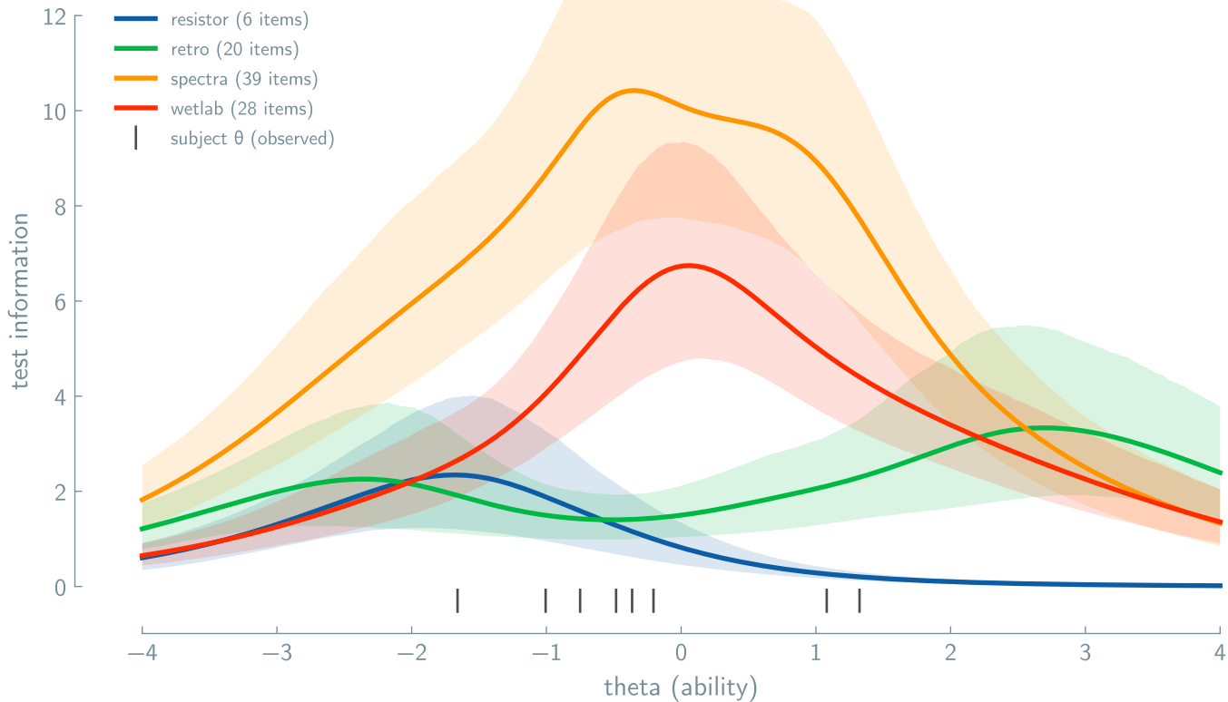
Test information by environment (89% ETI bands)
