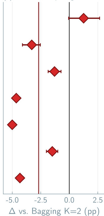
(b) matched-compute gain over bagging K=2
