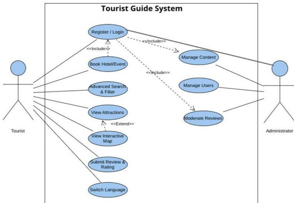
Figure 2: Use Case diagram of system
