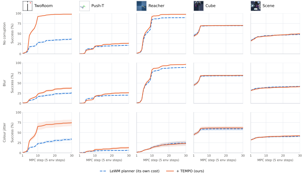
Figure 5: Test-time pixel corruptions: cumulative success versus MPC step, goal 75 steps ahead (30 steps = budget 150). Rows: condition; columns: environment. Dashed blue: the LeWM planner with its own cost; orange: the same planner + TEMPO (ours), on identical windows.
