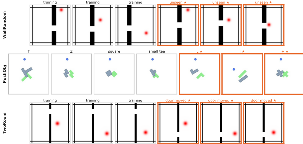
Figure 3: Training and test setups for the three generalisation families of Table 3. Unseen configurations are outlined in orange (*). WallRandom holds out wall and door positions outside every training range, PushObj holds out the L, I and + shapes, and TwoRoom moves the door to the opposite end of the wall.
