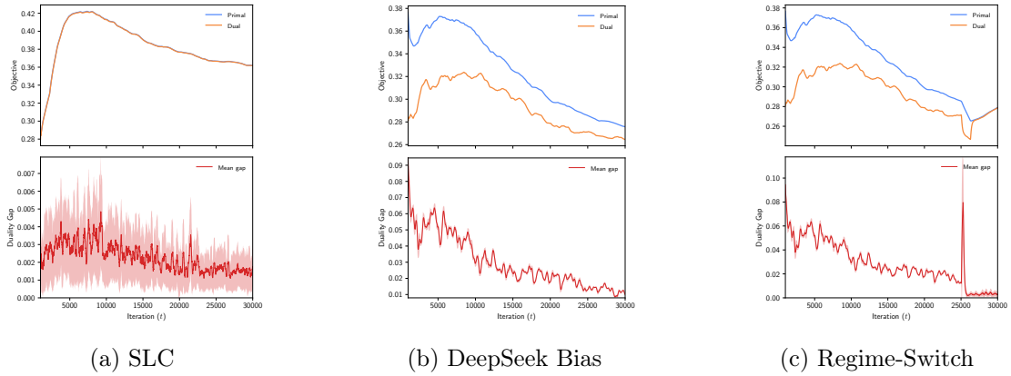
Figure 1: SLC Primal-Dual Convergence Dynamics (Layer 6, representing the terminal layer with peak congestion) . Trajectories of primal utility, dual objective value, and duality gap (smoothed via a rolling window-mean of 250 steps). (a) SLC establishes a stable saddle-point equilibrium with a duality gap below 0.085%. (b) DeepSeek baseline (proportional bias) exhibits wider variance and a higher final duality gap (3.64%). (c) The regime-switch experiment demonstrates rapid transient recovery when SLC is activated at step 25,000.
