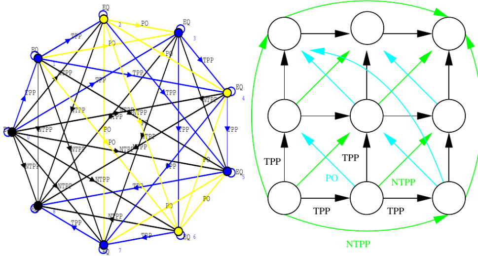
Figure 1: Wessel’s original \mathcal{ALCI}_{RCC8} grid construction, reproduced directly from report7.pdf (2002/2003) , Figure 10 (Section 4.4.3): a complete-graph RCC8 “frame” (left) that is isomorphic to a 3 \times 3 grid (right) and extends to n \times n . Horizontal and vertical successors are TPP edges (the intended roles R_X, R_Y ); PO (cyan) and NTPP (green) are the induced diagonal and long-range relations. Such grid models exist —but, as the same report already argued, no concept term can enforce them. (The frame was found by a Lisp enumerator and rendered with CLIM under MCL, not drawn by hand.) The construction and the obstruction are Wessel’s, two decades before this AI-assisted work.
