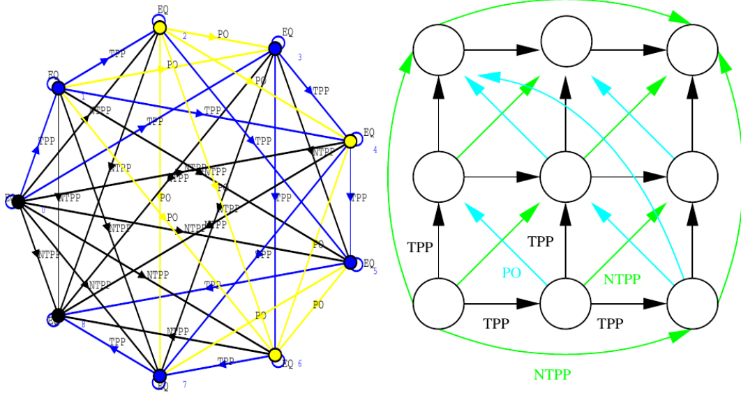
Figure 1: Wessel’s original \mathcal{ALCI}_{\text{RCC8}} grid construction, reproduced directly from report7.pdf (2002/2003), Figure 10 (Section 4.4.3): a complete-graph RCC8 “frame” (left) that is isomorphic to a 3 \times 3 grid (right) and extends to n \times n . Horizontal and vertical successors are TPP edges (the intended roles R_X , R_Y ); PO (cyan) and NTPP (green) are the induced diagonal and long-range relations. Such grid models exist —but, as the same report already argued, no concept term can enforce them. The construction and the obstruction are the human author’s, two decades before this AI-assisted work.
