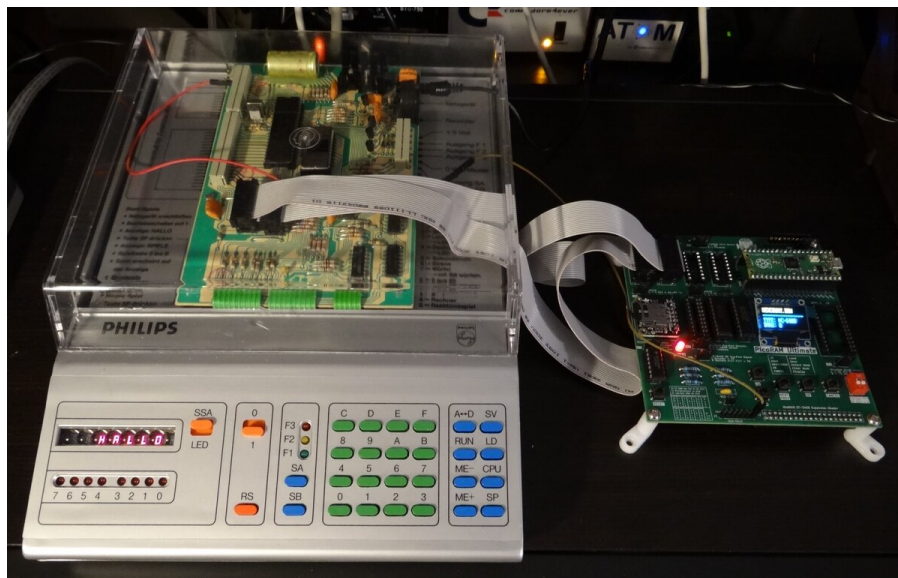
Figure 14. PicoRAM Ultimate (right) connected to the Philips MasterLab — it plugs directly into the machine's two 2114 SRAM sockets via the ribbon cable; the MasterLab's display shows its "HALLO" power-up greeting [32].
