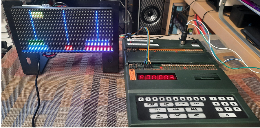
Figure 9. The real rig: a Kosmos CP1 (right) driving a 64 \times 32 RGB LED matrix (left) mid-solve, linked by the four-bit move protocol over jumper wires. The 8049-based 1983 trainer streams each Hanoi move to an Arduino Mega 2560, which renders the disks on the panel; the program itself was loaded through the CP1's cassette input as a WAV [40].
