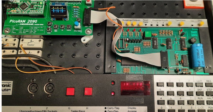
Figure 4. The first working Tic-Tac-Toe for the Microtronic, running on the PicoRAM 2090-extended machine: the 3 \times 3 grid is drawn on PicoRAM's OLED display (top left), with spoken moves and — for the human-first game — a new from-scratch board-scanning AI [14].
