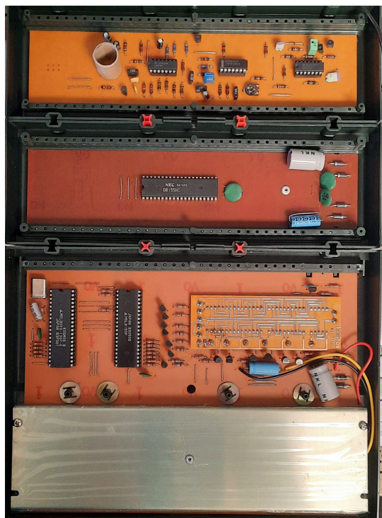
Figure 8. Inside the CP1 and its two stacked expansion modules (on the Kosmos construction rails). Bottom — the CP1 main board: the mask-programmed Intel 8049 microcontroller (here an M5L8049, marked "KOSMOS B") and an 8155 (M5L8155P) for RAM and I/O, above the orange keypad-matrix PCB and the shielded six-digit LED display. Middle — the CP3 memory expansion , built around a second 8155 (an NEC D8155HC). Top — the CP2 cassette interface , an analog board of op-amps and filters that generates and reads the cassette tones.
