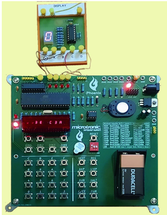
Figure 6. A new build running the original firmware: the Microtronic Phoenix [16].
