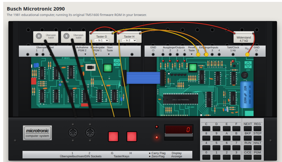
Figure 16. The Microtronic in the browser: the original firmware running in a JavaScript emulator [47].
