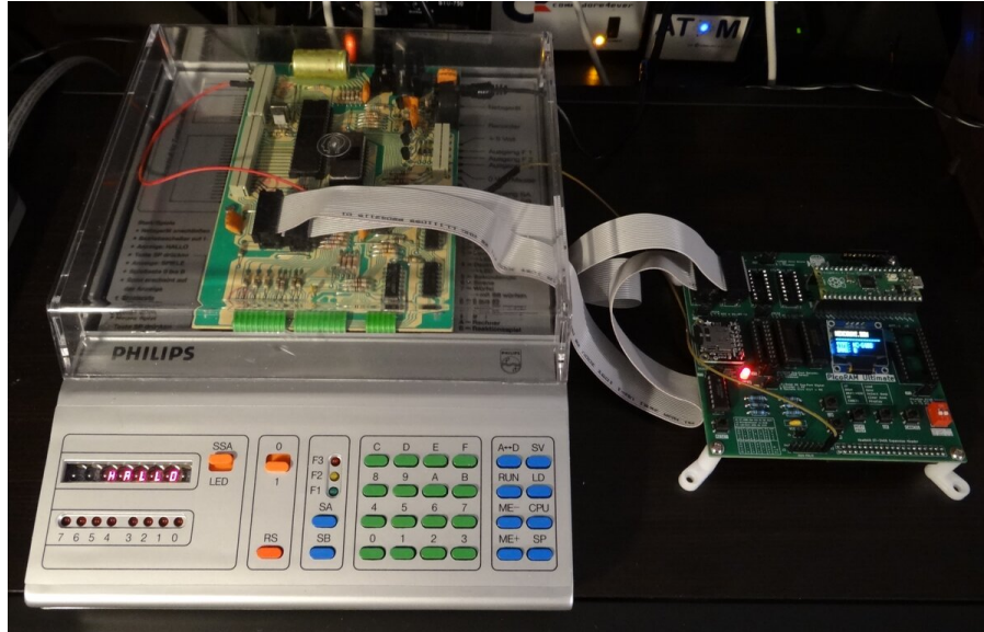
Figure 9. PicoRAM Ultimate (right) connected to the Philips MasterLab — it plugs directly into the machine's two 2114 SRAM sockets via the ribbon cable; the MasterLab's display shows its "HALLO" power-up greeting [31].
