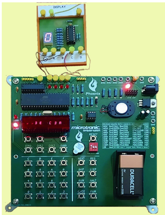
Figure 11. A new build running the original firmware: the Microtronic Phoenix [16].
