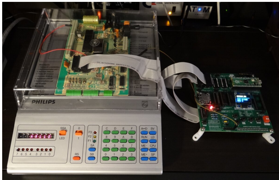
Figure 10. PicoRAM Ultimate (right) connected to the Philips MasterLab — it plugs directly into the machine's two 2114 SRAM sockets via the ribbon cable; the MasterLab's display shows its "HALLO" power-up greeting [31].
