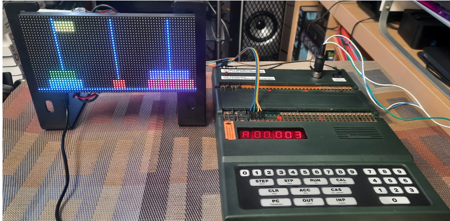
Figure 12. The real rig: a Kosmos CP1 (right) driving a 64 \times 32 RGB LED matrix (left) mid-solve, linked by the four-bit move protocol over jumper wires. The 8049-based 1983 trainer streams each Hanoi move to an Arduino Mega 2560, which renders the disks on the panel; the program itself was loaded through the CP1's cassette input as a WAV [40].
