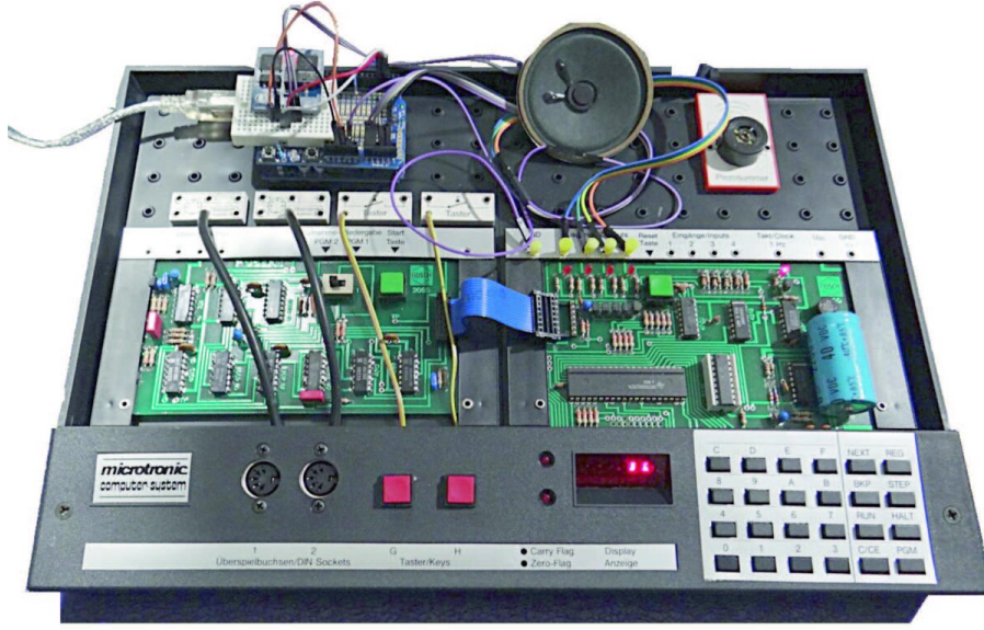
Figure 5. The Busch Microtronic with the original 2095 cassette interface and a DIY speech synthesizer.
