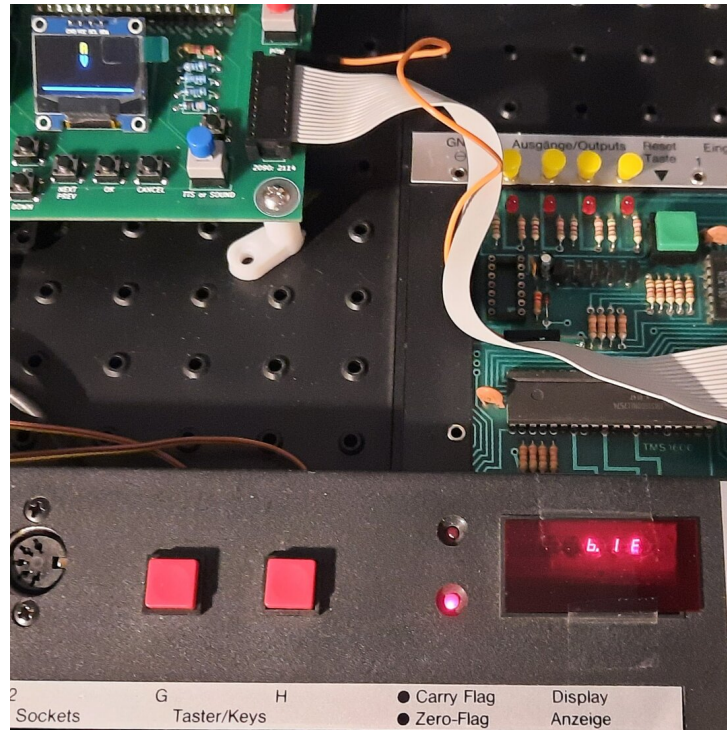
Figure 8. Lunar Lander — a wholly original game written from scratch for the PicoRAM 2090-extended Microtronic. The OLED (top left) is the cockpit window showing the descending lander; the red LED below shows the ALT / VEL / FUEL instruments [14].
