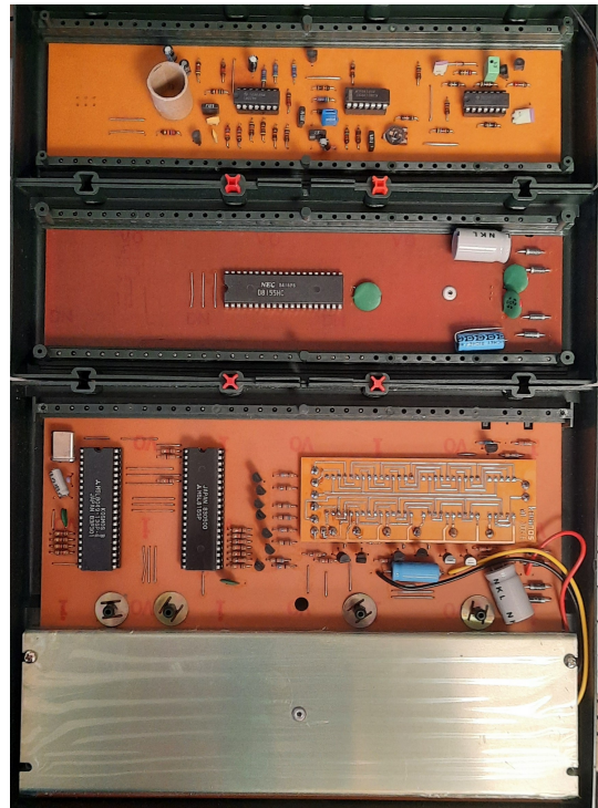
Figure 10. Inside the CP1 and its two stacked expansion modules (on the Kosmos construction rails). Bottom — the CP1 main board: the mask-programmed Intel 8049 microcontroller (here an M5L8049, marked "KOSMOS B") and an 8155 (M5L8155P) for RAM and I/O, above the orange keypad-matrix PCB and the shielded six-digit LED display. Middle — the CP3 memory expansion , built around a second 8155 (an NEC D8155HC). Top — the CP2 cassette interface , an analog board of op-amps and filters that generates and reads the cassette tones.
