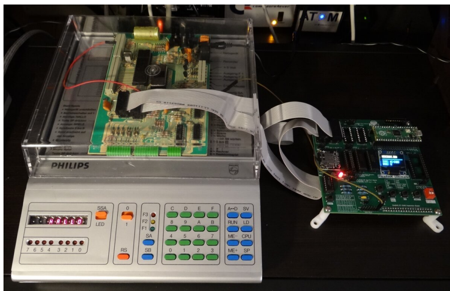
Figure 17. PicoRAM Ultimate (right) connected to the Philips MasterLab — it plugs directly into the machine's two 2114 SRAM sockets via the ribbon cable; the MasterLab's display shows its "HALLO" power-up greeting [32].
