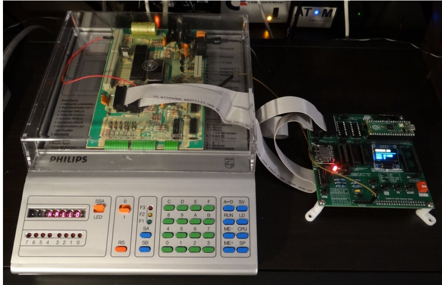
Figure 6. PicoRAM Ultimate (right) connected to the Philips MasterLab via the expansion bus; the MasterLab's display shows its "HALLO" power-up greeting [31].
