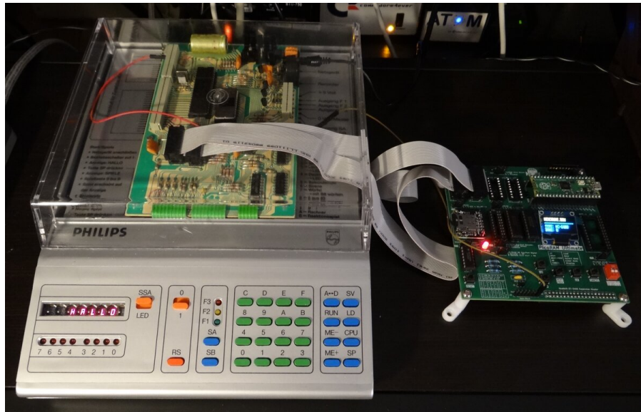
Figure 18. PicoRAM Ultimate (right) connected to the Philips MasterLab — it plugs directly into the machine's two 2114 SRAM sockets via the ribbon cable; the MasterLab's display shows its "HALLO" power-up greeting [34].
