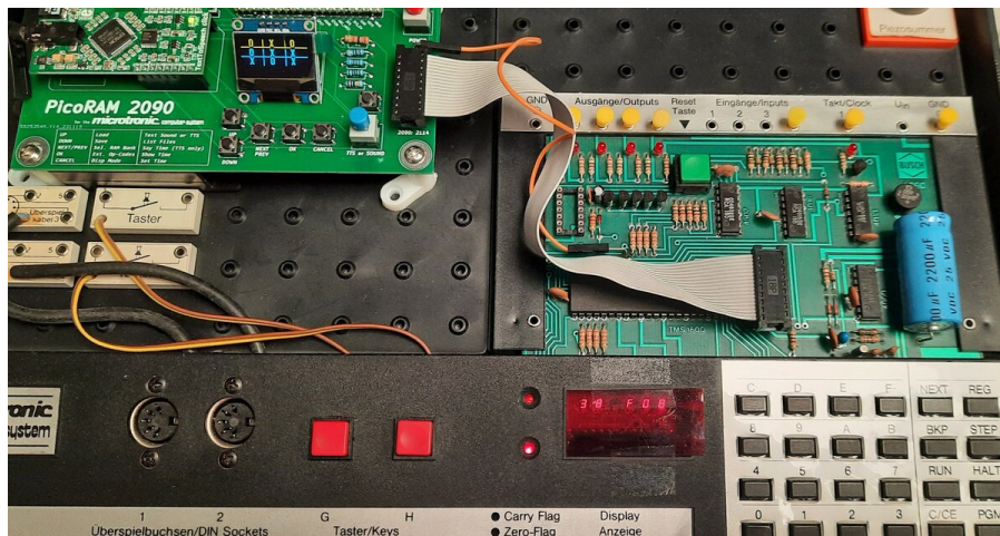
Figure 4. The first working Tic-Tac-Toe for the Microtronic, running on the PicoRAM 2090-extended machine: the 3×3 grid is drawn on PicoRAM’s OLED display (top left), with spoken moves and — for the human-first game — a new from-scratch board-scanning AI [14].
