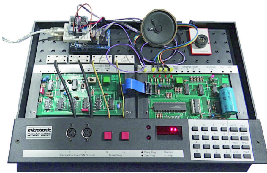
Figure 3. The Busch Microtronic with the original 2095 cassette interface and a DIY speech synthesizer.
