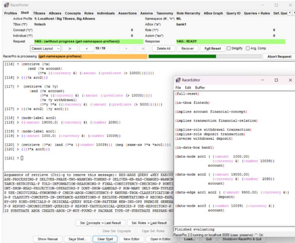
Figure 1: A property graph built and queried in RacerPro 2.0 (RacerPorter). Nodes acc1–acc3 and the deposit edge carry key–value property maps; nRQL filters on node and edge properties and traverses the deposit/withdrawal (inverse) edge, while node types ( account ) are OWL/DL concepts and edge labels are DL roles.
