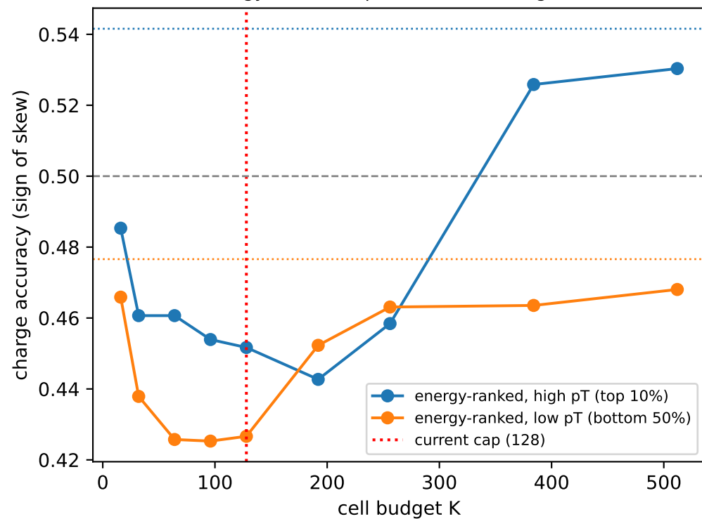
(a) Energy-ranked cap vs all-cells ceiling (dotted)
