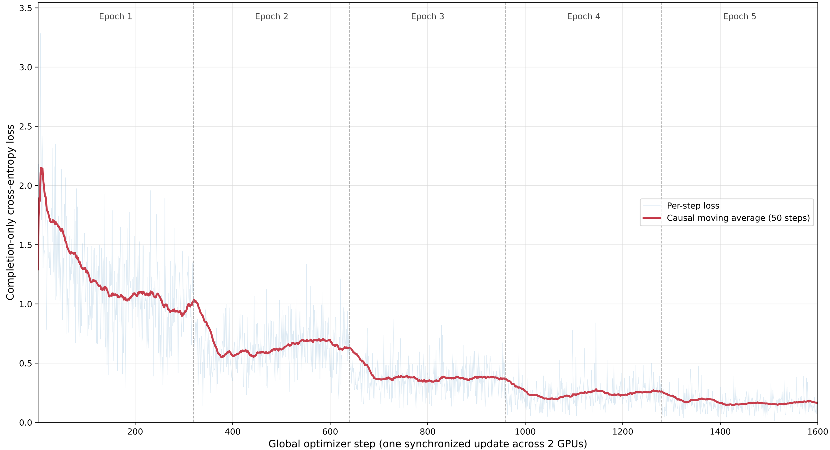
Qwen3-8B AppWorld Full-Parameter SFT Training Loss — 5 Epochs
