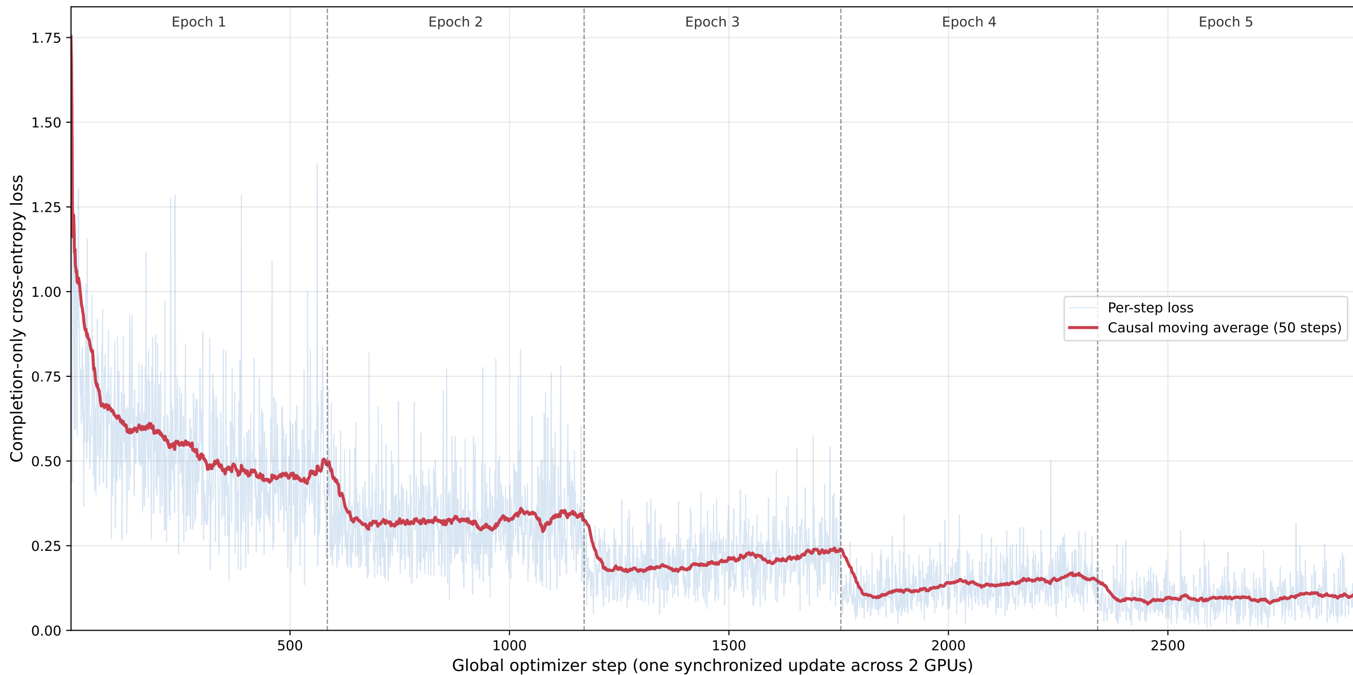
Qwen3-8B AppWorld Codex-RFT LoRA Training Loss — 5 Epochs
