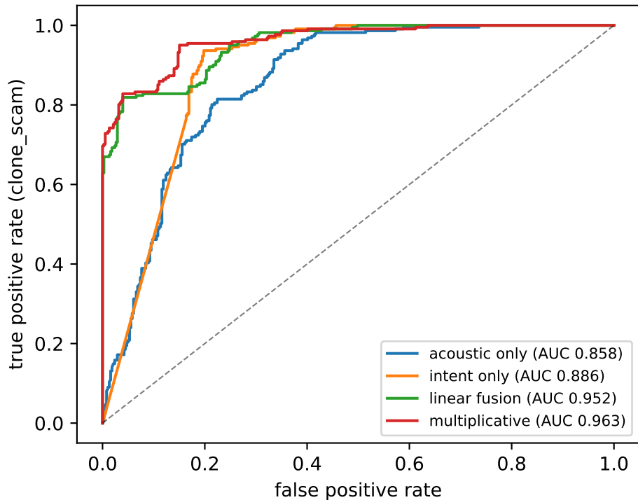
ROC on ASVspoof (m1)
