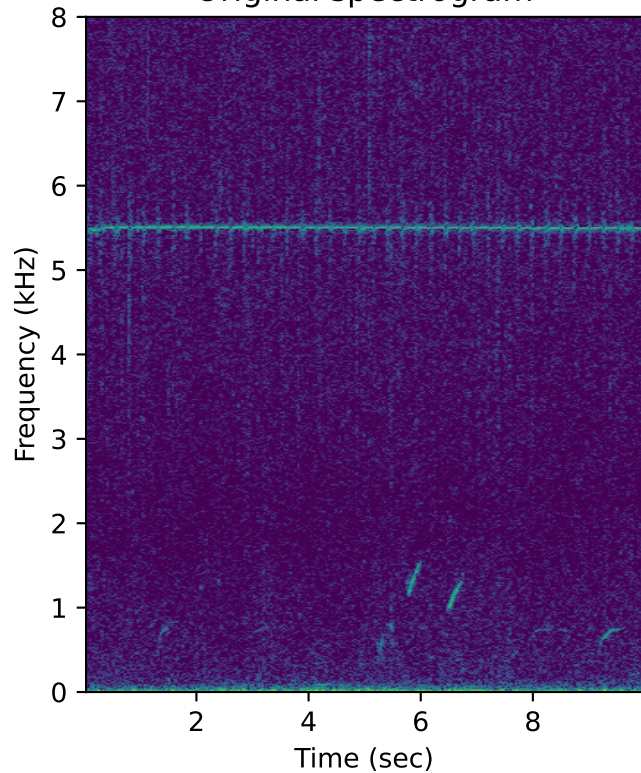
Original spectrogram
