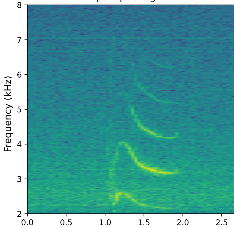
Input spectrogram
