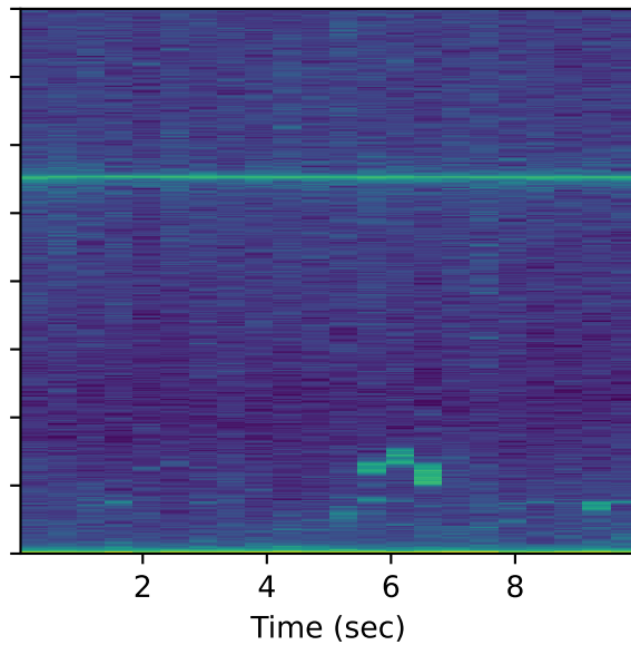
Max-pooled spectrogram
