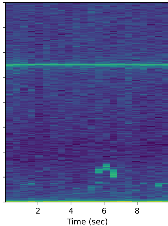
Max-pooled spectrogram
