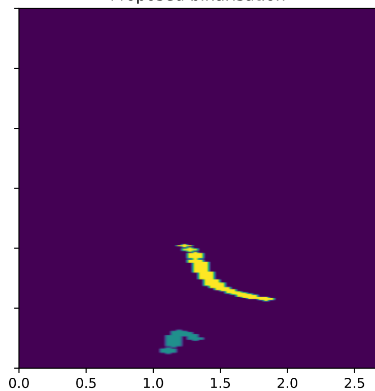
Proposed binarisation
