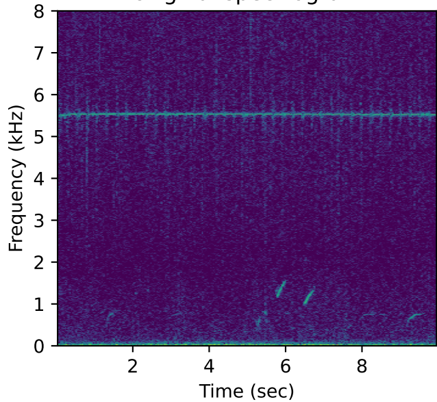
Original spectrogram
