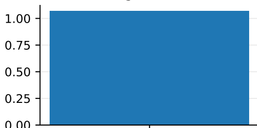
edges / idea
